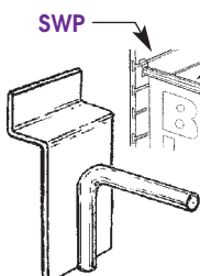
SWP SLAT WALL PEG 1/4"D x 1 1/2"Lg.
