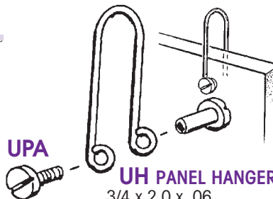
HC HANG-COIL 3/8" x 1 1/8" x .04 Nickel plated spring steel. Twist in place in foam boards and acoustical ceilings.
